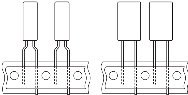
Pitch F = 5 mm. Case \text{ØD} \times L = 5 \times 11 and 8.2 \times 11 mm.
