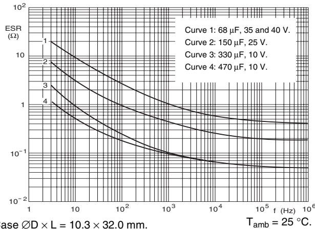
Fig.27 Typical ESR as a function of frequency.
