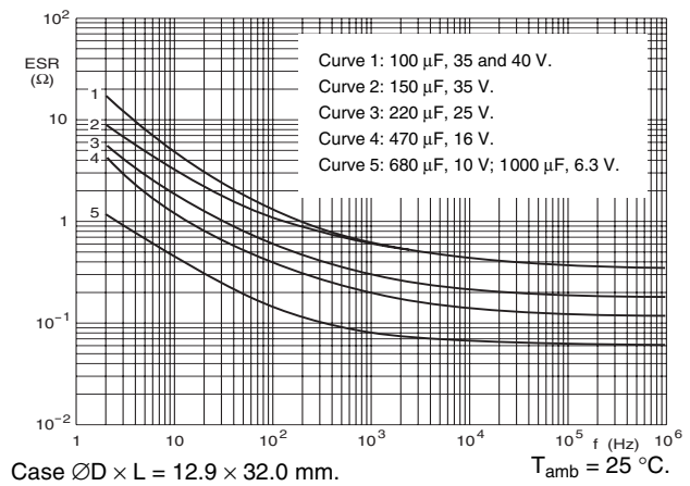
Fig.28 Typical ESR as a function of frequency.
